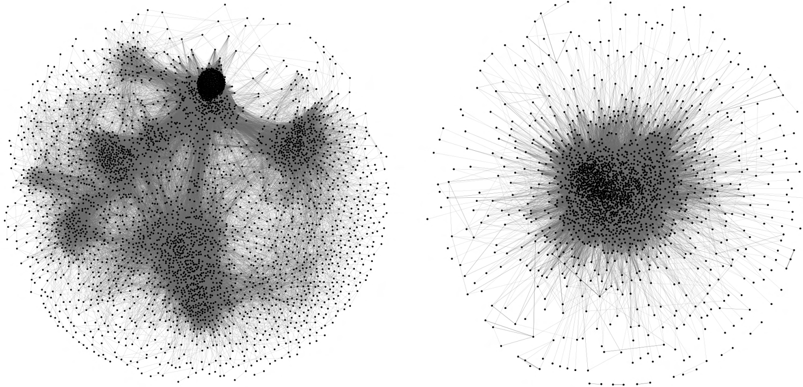
FIGURE 1: NETWORK VISUALIZATION
