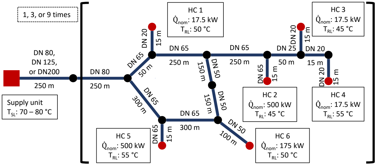
Figure 3. Layout of the demonstration network with the main parameters: Nominal heat load and constant return line temperature of HCs (HC 1 to HC 6), supply line temperature at the supply unit and nominal diameter and length for the pipe segments. Simulations were run for different network sizes where the network part in brackets exists 1, 3 or 9 times after the first pipe.
