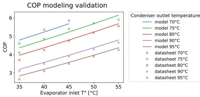
Figure 14. Heat pump COP validation
