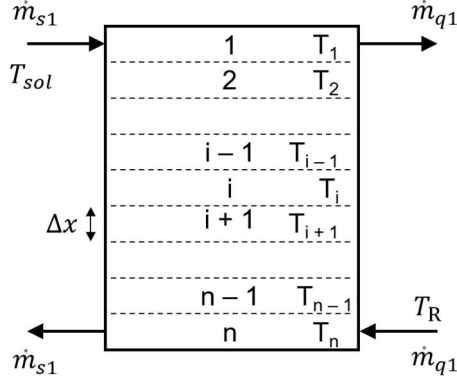
Figure 6. Spatial discretization of TTES (Scolan et al. 2020)
