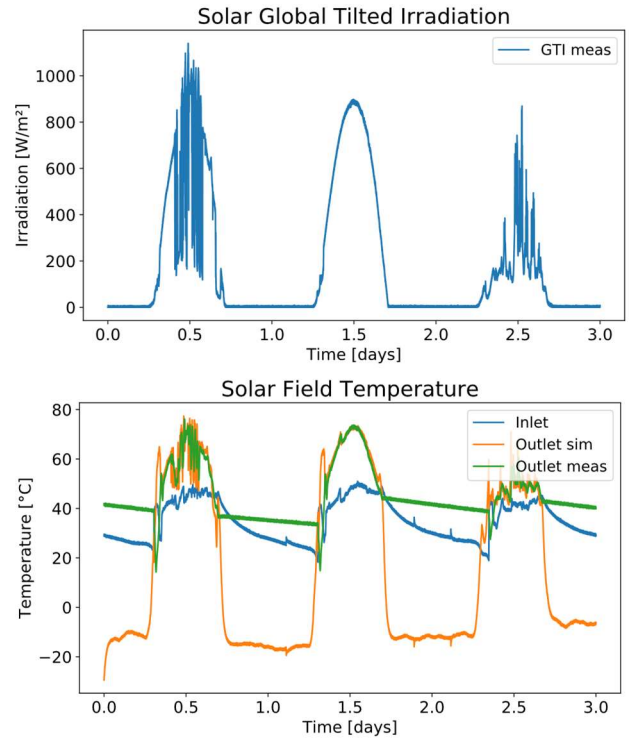
Figure 9. Solar field validation
