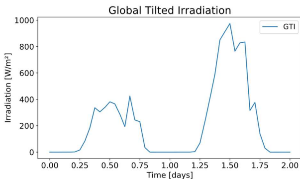
Figure 15. Full plant simulation - Global Tilted Irradiation
