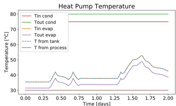
Figure 19. Full plant simulation - Heat pump temperatures
