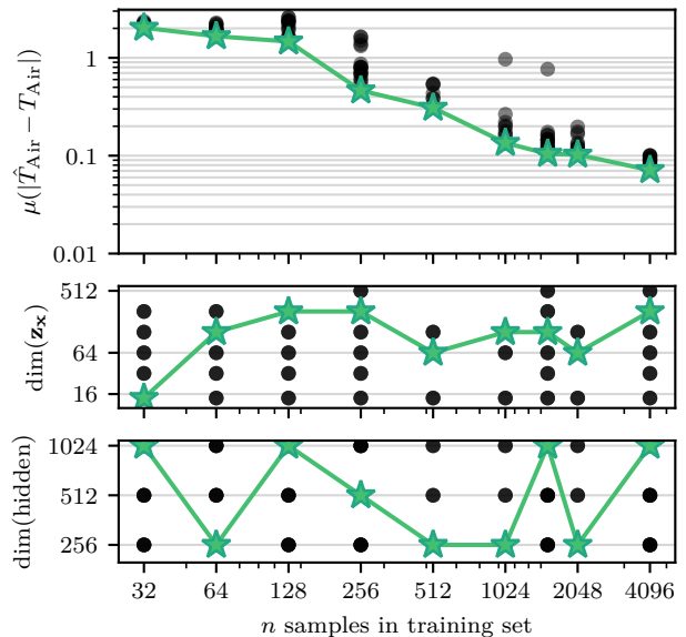
Figure 6. Hyperparameter variation (latent space dimension \dim \mathbf{z}_x and dimension of hidden layers) over training sets with different number of samples n , tested with same uniformly sampled test set, all within [\theta_-, \theta_+] . The best-performing model for each training dataset size is marked by a star. (training performed for day 8-16 of identification timeframe)
