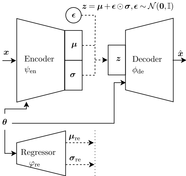
Figure 3. Physics-Enhanced Latent Space Variational Autoencoder (PELS-VAE). The time-series \mathbf{x} is introduced to the Encoder \psi_{\text{en}} , which transforms it to a latent-space distribution with mean \boldsymbol{\mu} and variance \boldsymbol{\sigma} , which can be decoded by the Decoder \phi_{\text{de}} by sampling \mathbf{z} with the auxiliary Gaussian variable \boldsymbol{\epsilon} to reconstruct the time-series as \hat{\mathbf{x}} = \frac{1}{L} \sum^L \phi_{\text{de}}(\mathbf{z}) . The Regressor \varphi_{\text{re}} is trained simultaneously to predict the mean and variance of the latent space distribution. As in (Martínez-Palomera, Bloom, and Abrahams 2020), the physical parameters \boldsymbol{\theta} are introduced to all models. (Zhang and Mikelsons 2022)
