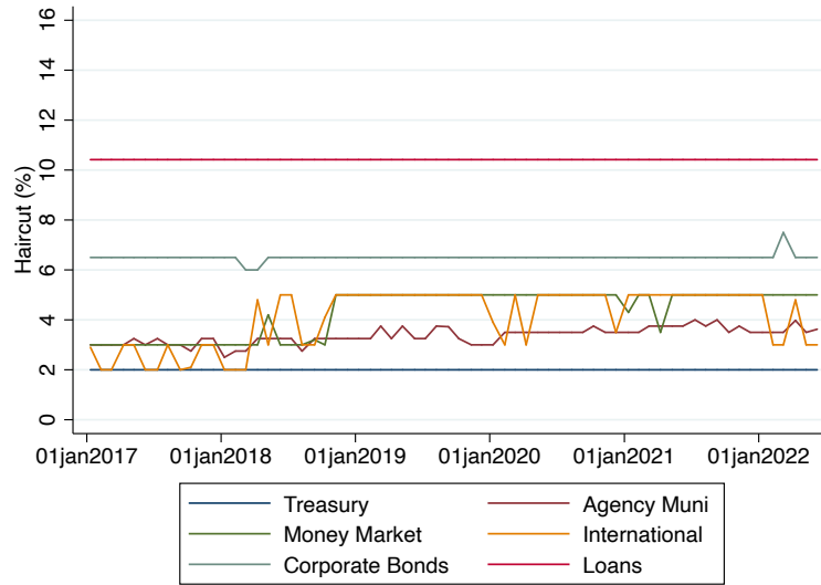
Figure 4: Liquidation Discounts
