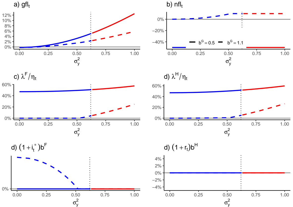
Figure E.1: Comparative statics of \sigma_y^2 - continued
