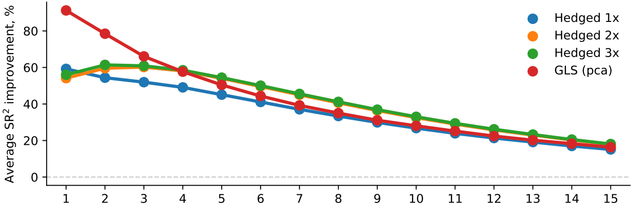
FIGURE I: In-sample maximum squared Sharpe ratio improvement due to iterative hedging of OLS factors. The plot shows improvement, in %, of annualized average in-sample maximum squared Sharpe ratio of hedged OLS factors relative to unhedged factors, for all models with a constant and 1–15 additional factors. We hedge the factors up to three times. We also report performance of the GLS factors which use the sample conditional covariance matrix of individual stock returns estimated using the rolling PCA procedure outlined in Section V.B. For each number of factors on the x -axis, results are averaged across 10,000 models with this number of factors randomly drawn from the set of all factors.
